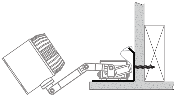
VERTICAL MOUNTING
