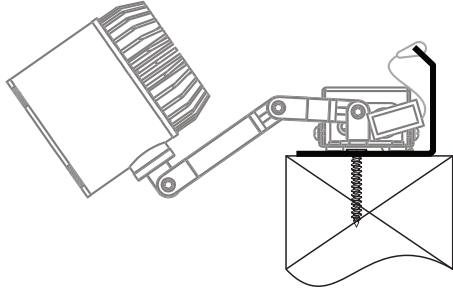
HORIZONTAL MOUNTING
